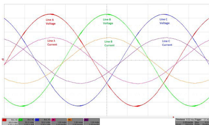
Figure 5. 60Hz, 50% Load, 2 msec/div Line Voltage: 50 V/div Line Current 1 A/div
