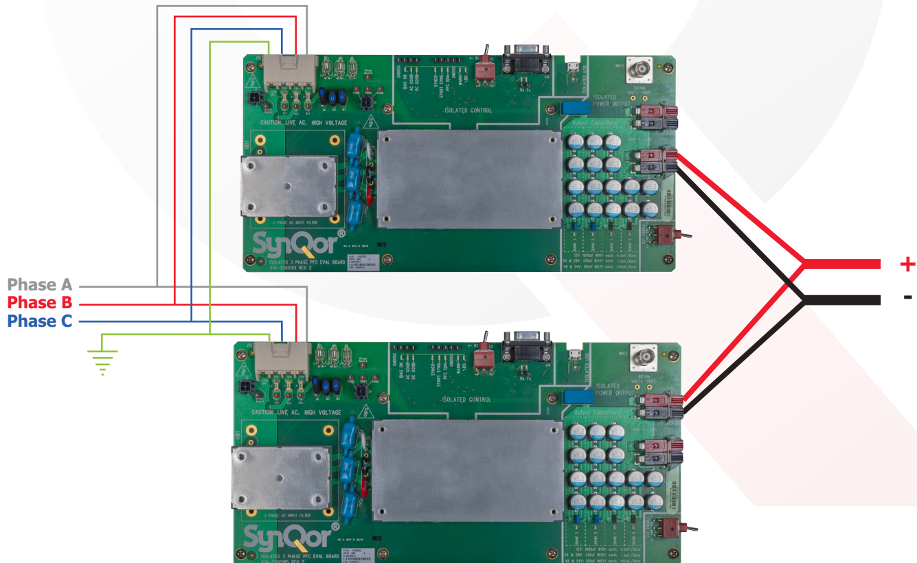
Figure 9. Simplified paralleling diagram of two AeroQor 3-Phase Isolated PFC EVAL-KIT droop share option boards powered from a single source.
