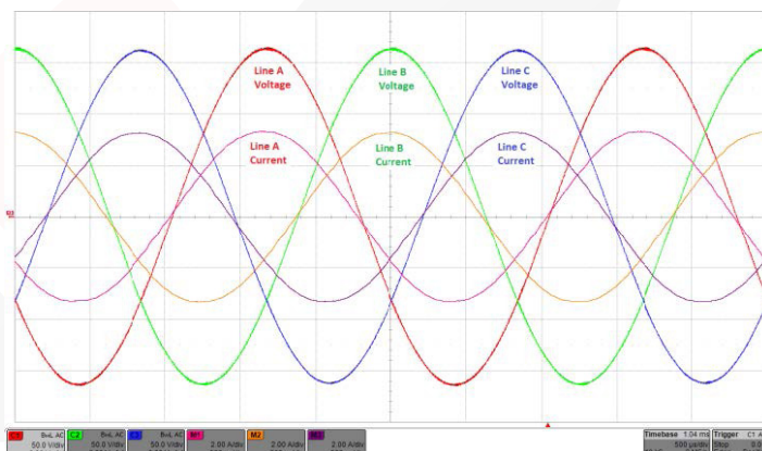
Figure 8. 400Hz, Full Load, 0.5 msec/div Line Voltage: 50 V/div Line Current 2 A/div
