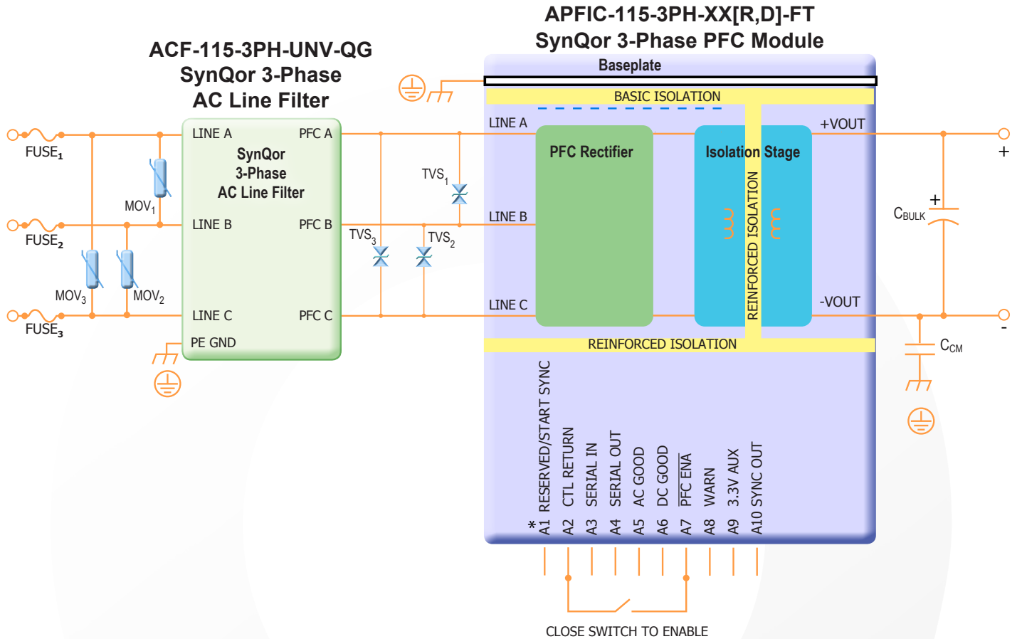
Figure 1: Typical connection diagram for the APFIC-115-3PH-XX[R,D]-FT 3-Phase AC-DC converter. * Reserved for Regulated Module START SYNC for Droop Module.
