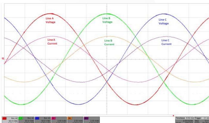
Figure 6. 60Hz, Full Load, 2 msec/div Line Voltage: 50 V/div Line Current 2 A/div
